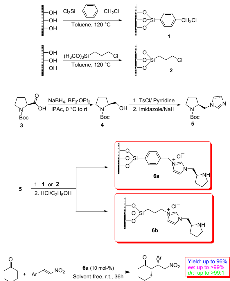
Scheme 1. Synthesis of silica gel supported pyrrolidine-based chiral ionic liquid and its application in asymmetric Michael addition to nitrostyrenes.
